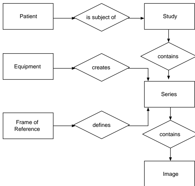
Figure 1: The DICOM composite instance IOD information model.
