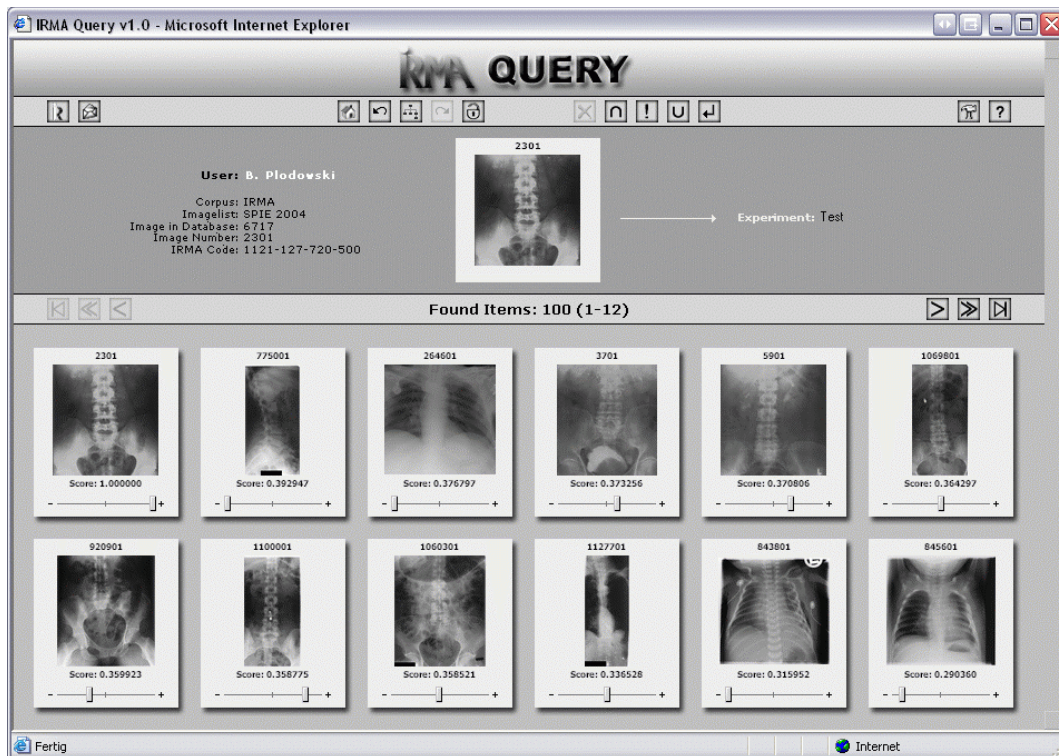
Figure 4: Query refinement stage of a web-based CBIR GUI
