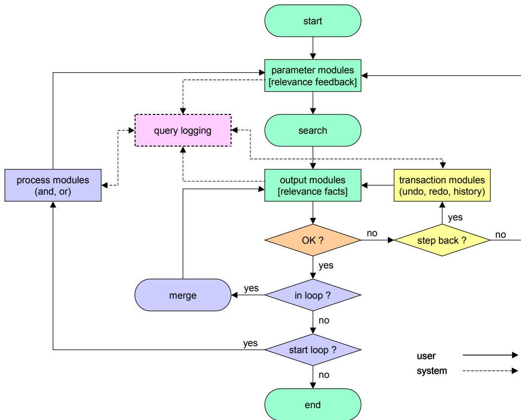
Figure 1: Flowchart of extended query refinement
