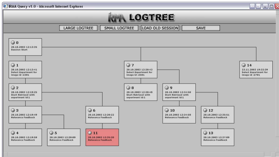
Figure 5: Screenshot of a web-based GUI to select and restore previous system stages
